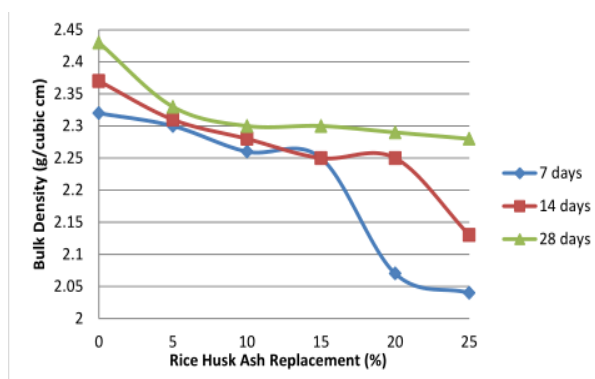
Fig.3: Effect of RHA content on Bulk Density of Concrete at different curing age [12].
