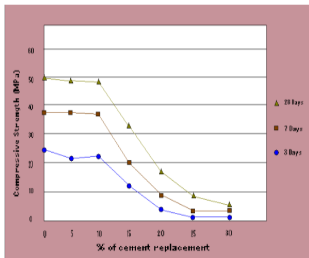
Fig.2: Effect of RHA content on Compressive Strength of Concrete at different curing age [10].
