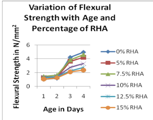
Fig.4: Variation of Flexural with age and percentage of RHA [13]
