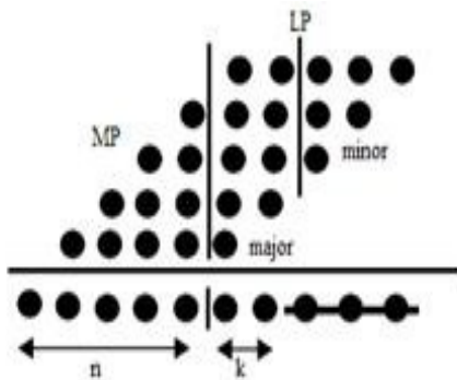
Fig.6. Partial-products matrix of a 5x5 bit multiplier.
