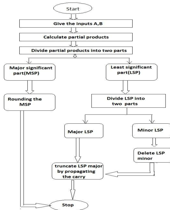
Fig.7. Truncated Flow Chart.
