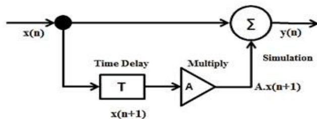
Fig.1. Block diagram of a Simple Digital Filter.
