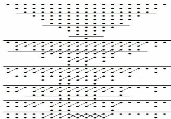
Fig.8. Modified Wallace reduction block diagram.
