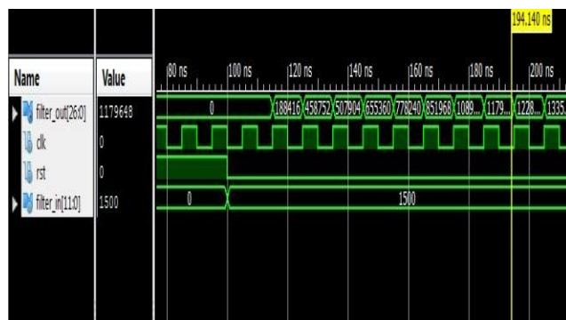
Fig. 15. Waveform.
