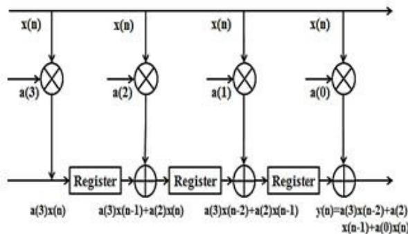
Fig.2. Direct Form FIR Filter Architecture.
