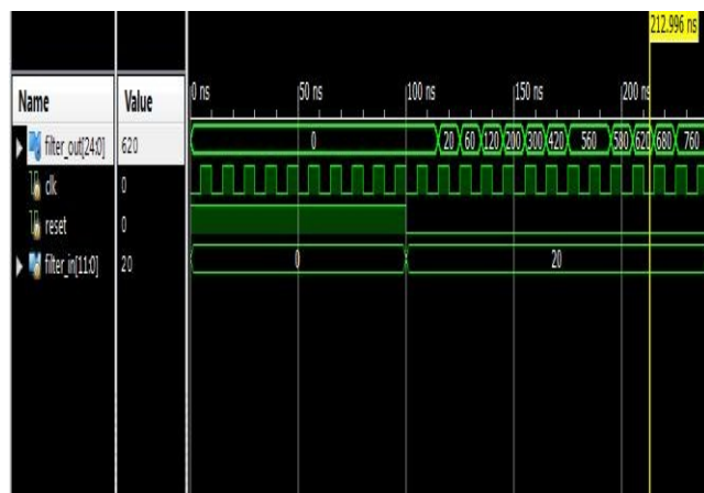
Fig.12. Waveform.
