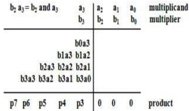
Fig.5. 4x4 bit Binary Multiplication with truncation degree T=3 .
