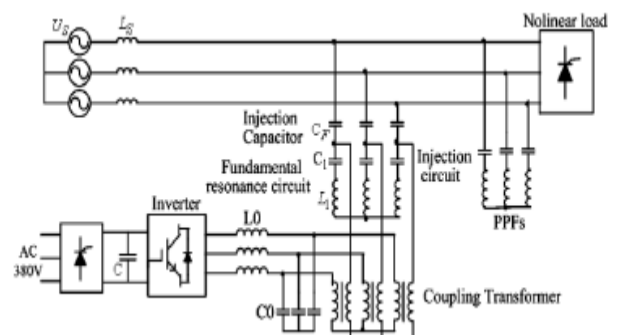
Fig.2 Topology of the novel HAPF
