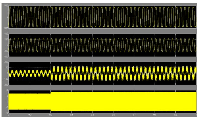
Fig. 7 Simulation results of steady-state compensation. (a) Simulation results with the conventional generalized integral controller. (b) Simulation results with the proposed fuzzy controller
