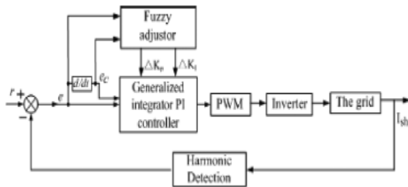
Fig.4 Configuration of the adaptive fuzzy dividing frequency controller
