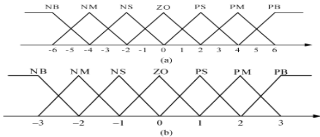
Fig.6 Membership functions of the fuzzy variable. (a) Membership function of e(k) and e_c(k) (b) Membership function of \Delta K_P and \Delta K_I .
