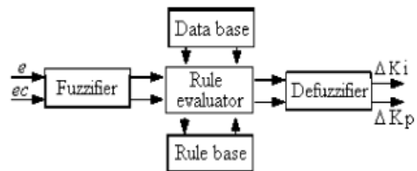
Fig.5 Block diagram of the fuzzy adjustor unit
