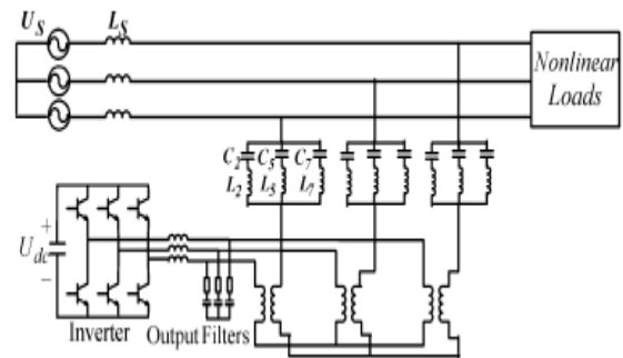
Fig.1 Topology of the shunt hybrid APF
