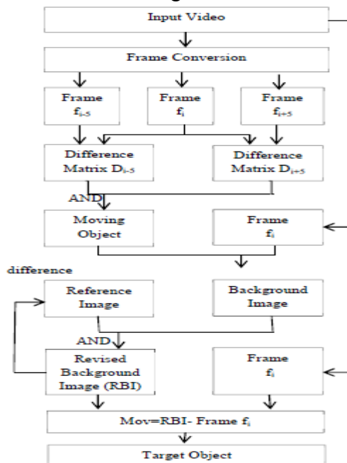
Figure 3: Flow Chart of BSFD Algorithm The formula of the moving target detection algorithms based on the dynamic background as follows
