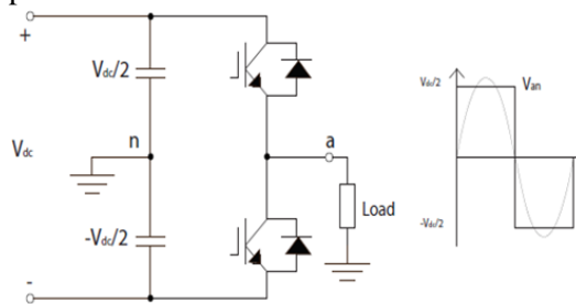
Fig. 1: Traditional single phase inverter
