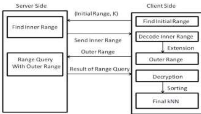
Fig. 3. Procedure of the KNN-R algorithm.
