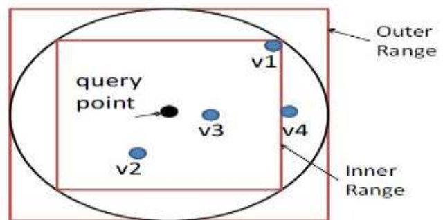
Fig. 2. Illustration for kNN-R Algorithm when k = 3.
