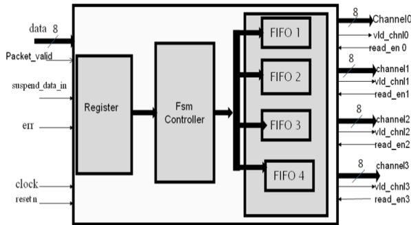
Figure2: Internal Structure of Protocol
