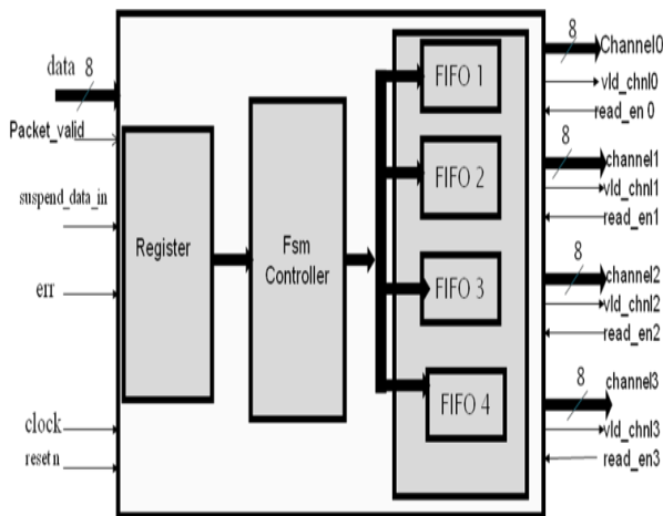
Figure2: Internal Structure of Protocol
