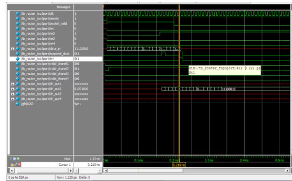
Figure 7: Simulation Results of Router Protocol-
