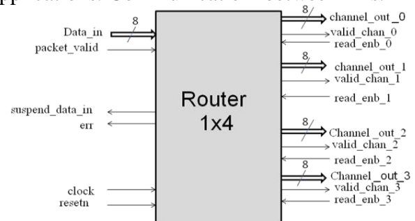
Figure1: Block Diagram of Router Protocol
