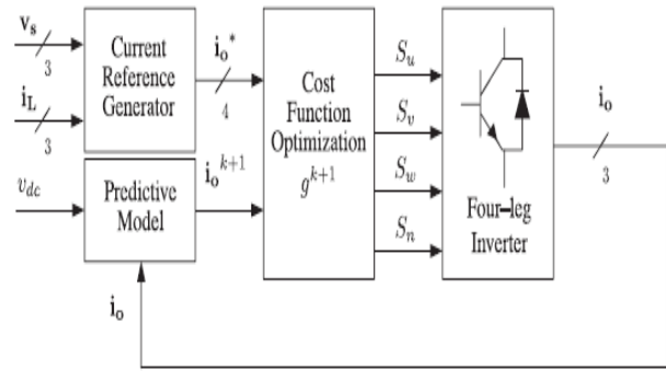
Fig. 4. Proposed predictive digital current control block diagram.
