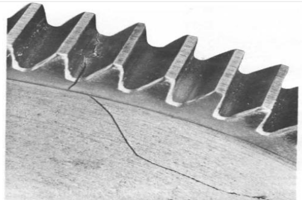
Fig.3 failure by cracking
