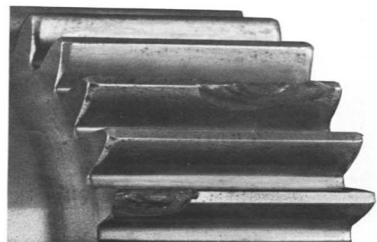
Fig.4 Gear teeth fracture
