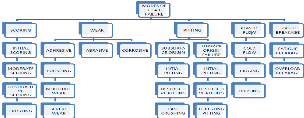
Fig. 1 Different modes of failure
