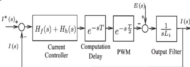
Fig-3: Current control loop diagram
