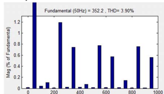
Fig a. PCC voltage of phase “a”
