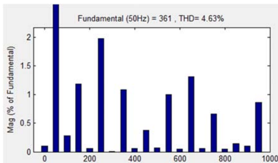
Fig d. PCC voltage of phase "a"
