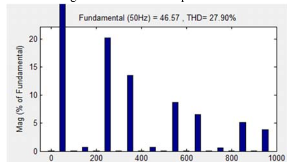
Fig c. load current of phase “a”
