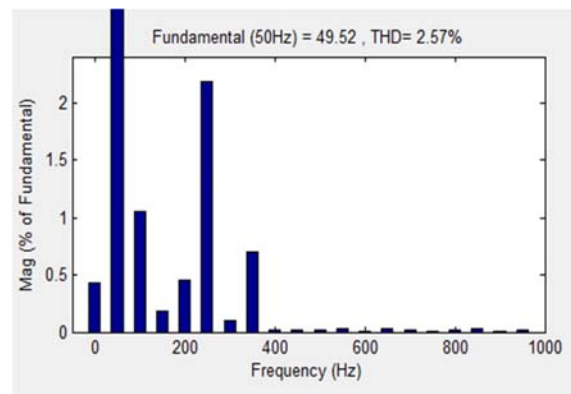
fig g. load current of phase "a"
