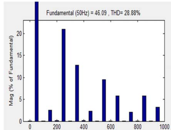
Fig f. load current of phase "a"
