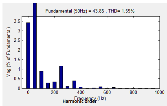
Fig k. Source current of phase “a”
