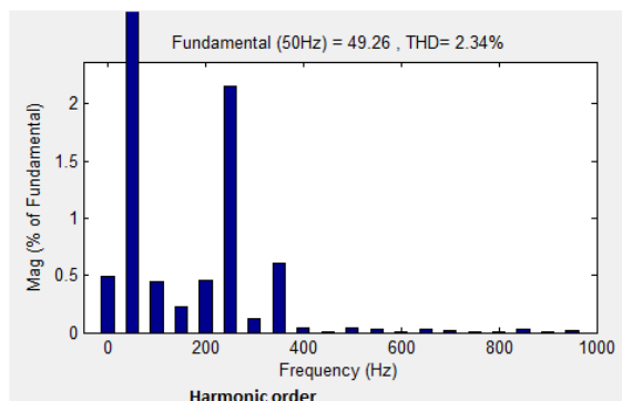
fig l. Load current of phase “a”
