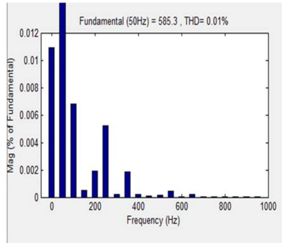
Fig i. PCC voltage of phase a “ v_{sa} ”
