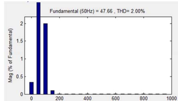
Fig b. source current of phase “a”
