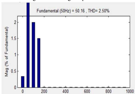
Fig e. source current of phase "a"
