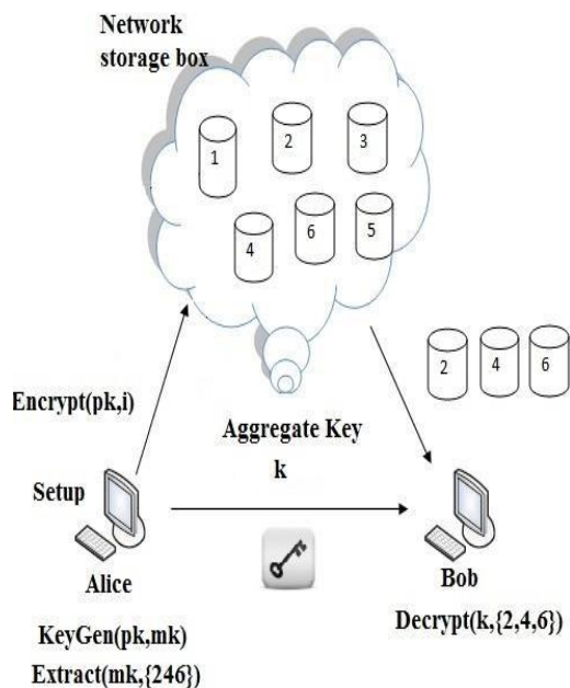
Fig 2 Use of KAC for data sharing
