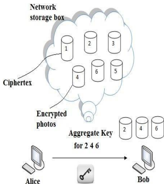
Fig 1 File sharing between Alice and Bob
