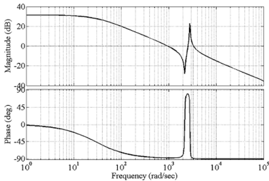
Fig.5. Frequency response \frac{\Delta V_{dc1}(s)}{\Delta \delta_1(s)} at i'_{q0} = 1.02 p.u., \delta_1 = -0.9^0, \delta_2 = 178.9^0 R_1 = 80 p.u., R_2 = 60 p.u.
