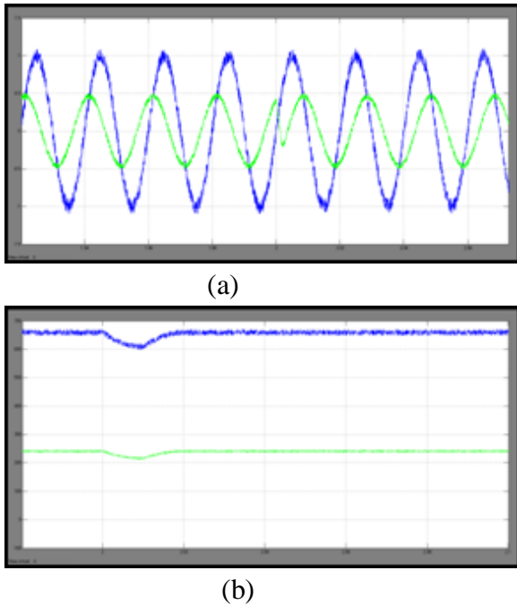
Fig. 7. Reactive power control. (a) Source voltage and inverter current. (b) DC-link voltages of two inverters.
