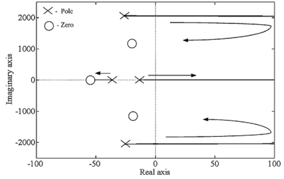
Fig.6. Frequency response \frac{\Delta V_{dc1}(s)}{\Delta \delta_1(s)} at i'_{q0} = -0.75 p.u., \delta_1 = 0.57^0, \delta_2 = -179.6^0 R_1 = 80 p.u., R_2 = 60 p.u.
