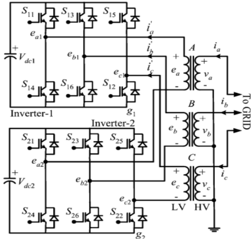
Fig. 2. Cascaded two-level inverter-based multilevel STATCOM.
