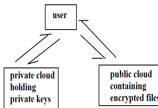
Fig1: an overview of Authorized Deduplication
