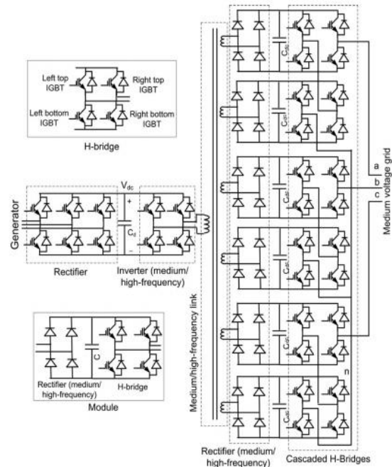
Fig.3. Detailed power conversion circuit
