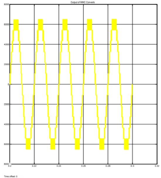
Fig.10. MATLAB based simulation output voltage waveform diagram of proposed system
