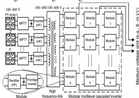
Fig.2. Proposed medium-voltage PV inverter system
