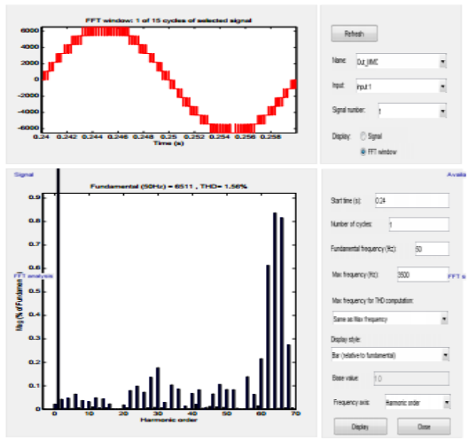
Fig.9. FFT Analysis window diagram
