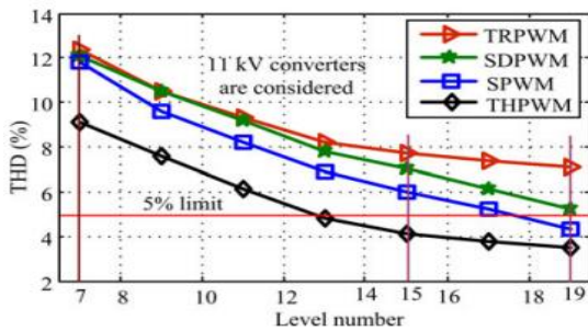
Fig. 5. Calculated THD at different number of levels ranging from 7-level to
