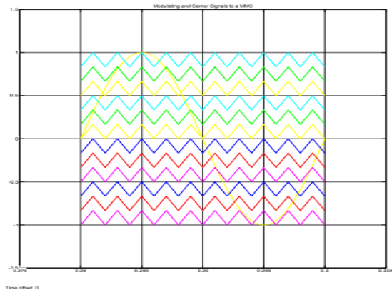
Fig.8. shows the MATLAB based simulation carrier signal
