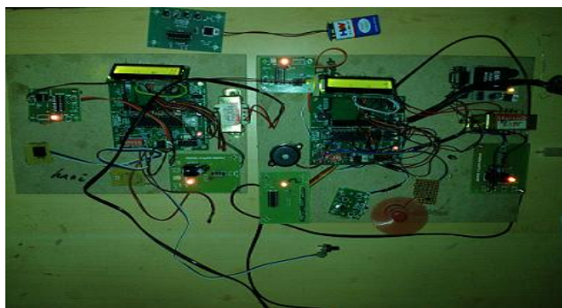
(a) Slave and master communication using can protocol
