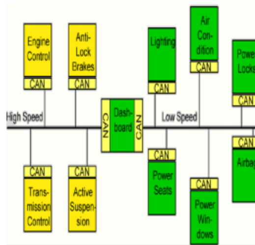
Figure 3.1 General diagram of implementation of CAN Protocol
