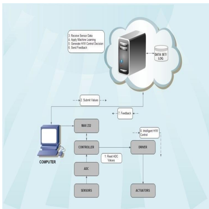
Figure :2 Schematic Block Diagram
