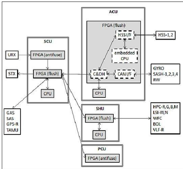
Figure 1: Overall System structure connecting different sensing units
