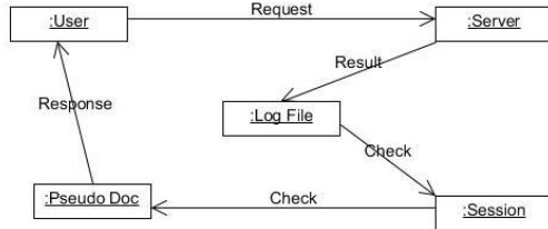
Figure : Collaboration Diagram
