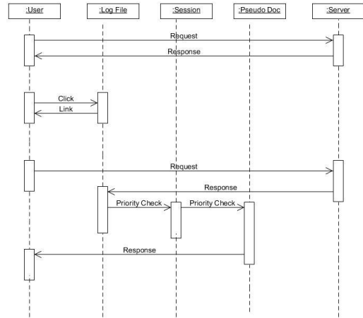
Figure : Sequence Diagram
