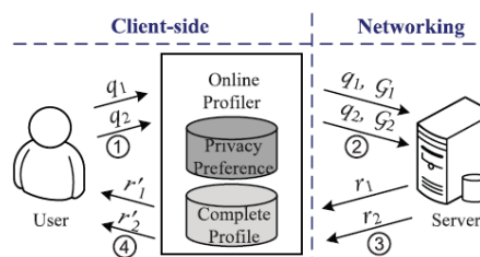
Figure 2: System Architecture
