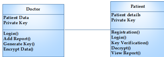
Figure 5: Class Diagram
