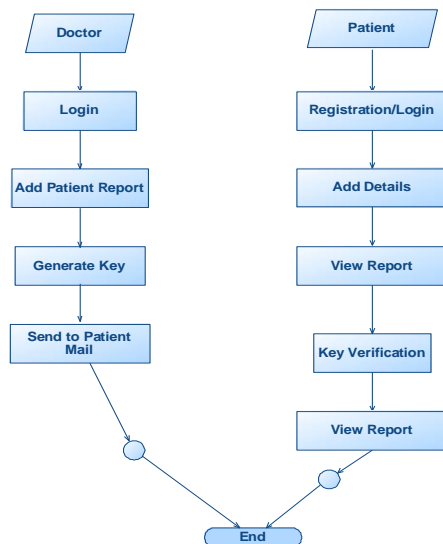
Figure 3: Data Flow Diagram UML DIAGRAMS
