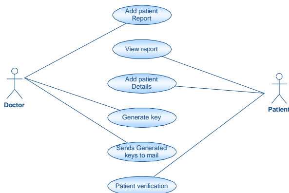
Figure 4: Use Case Diagram
