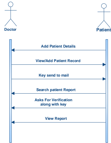
Figure 6: Sequence Diagram
