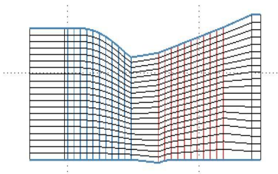
Fig 4.computational domain of the test turbine build
