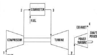
Fig 1. Gas Turbine Simple Open Cycle
