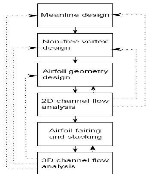
Fig 3. The aerodynamic design process.
