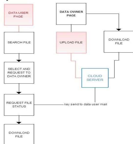
Figure1: Proposed Approach
