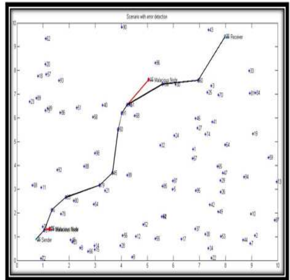
Fig. 10: Retraced Path after Fault Detection
