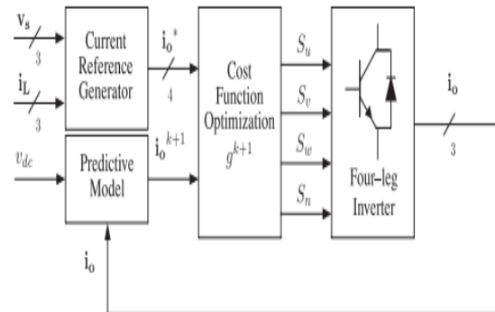
Fig. 2. Proposed predictive digital current control block diagram
