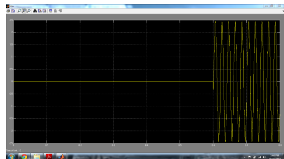
Fig.9. MATLAB based simulation of the proposed control scheme - Active power filter neutral current
