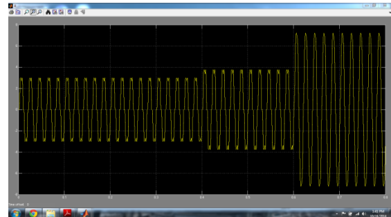
Fig.8. MATLAB based simulation of the proposed control scheme Load Current
