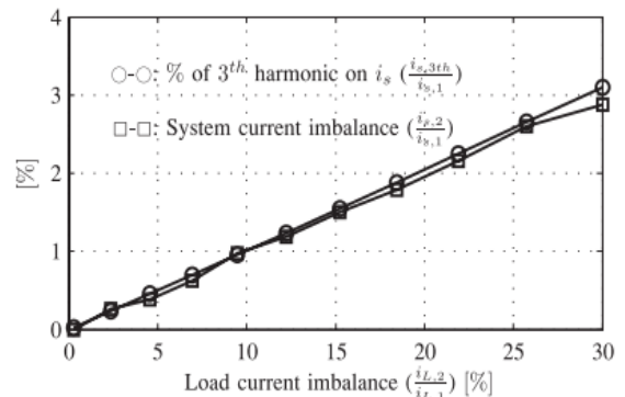
Fig. 4. Relationship between permissible unbalance load currents, the corresponding third-order harmonic content,
