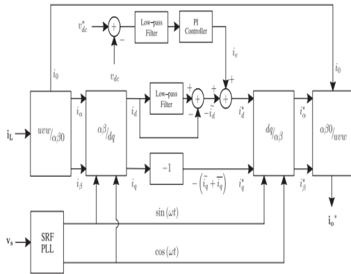
Fig.3. dq-based current reference generator block diagram.
