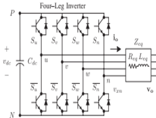
Fig. 1. Two-level four-leg PWM-VSI topology
