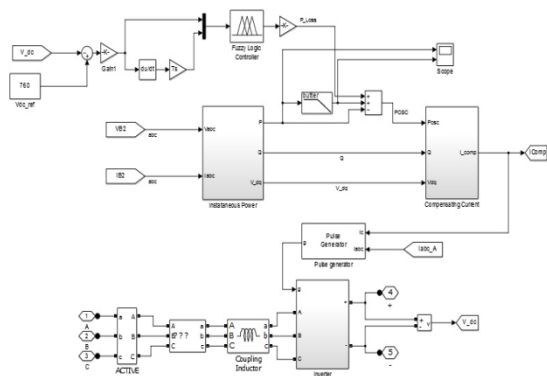
Fig.6. MATLAB based simulation diagram of proposed system with masked blocks
