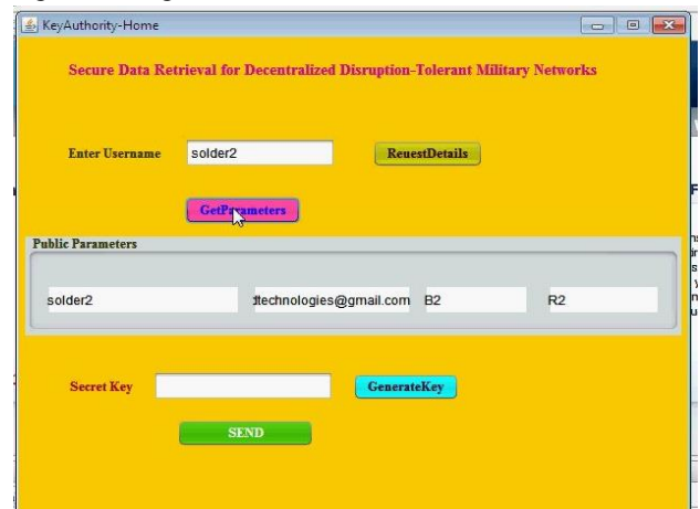
Fig 5: Revising Files
