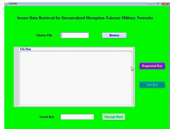
Fig 4 Sending Files
