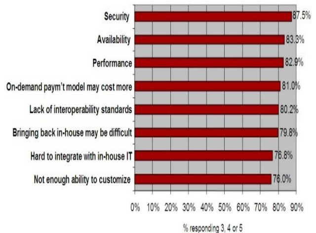
Fig.3. Ranking of facing problems during Cloud Computing platform construction
