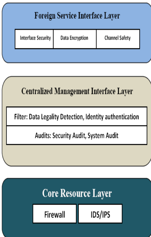
Fig.2. Security Issues at different layers of Cloud
