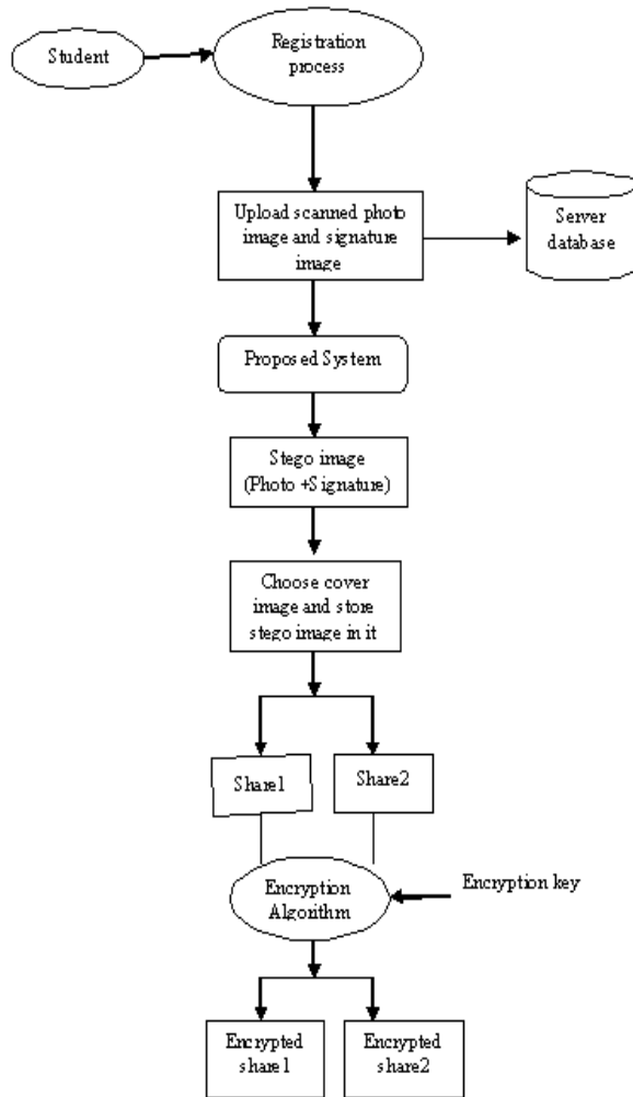
Fig2. Encryption at server side
