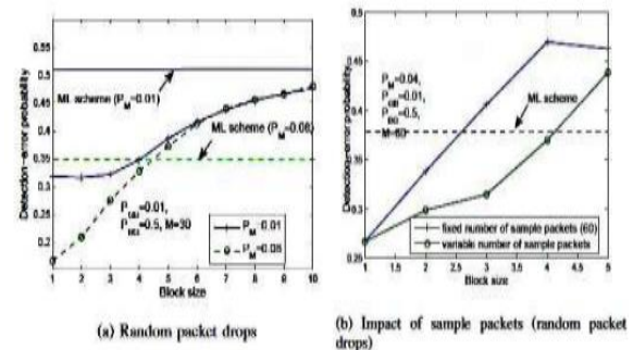
Fig. 5. Detection accuracy of block-based algorithms
