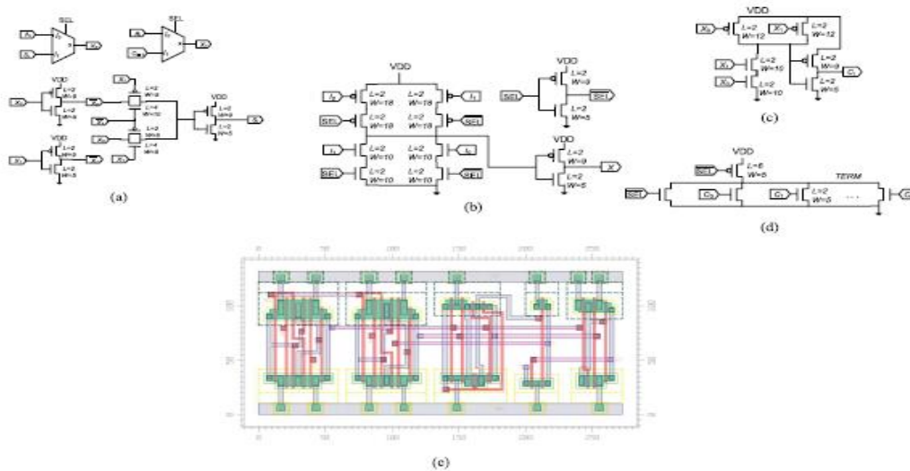
Fig. 3. CMOS implementation of PASTA. (a) Single-bit sum module. (b) 2 \times 1 MUX for the 1 bit adder. (c) Single-bit carry module. (d) Completion signal detection circuit.
