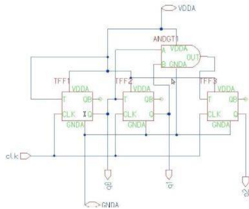
Fig. 3. Schematic of a 3-bit Synchronous Counter of Proposed Flip Flop
