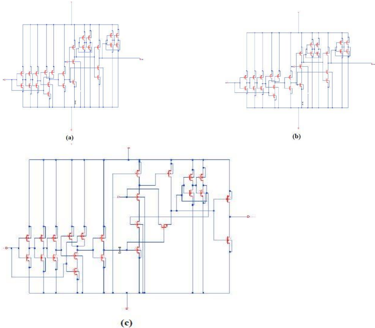
Fig. 1. Flip Flop Design (a) ep-DCO , (b) CDFF and (c) Base Paper Model Flip Flop
