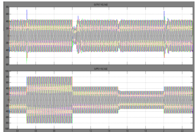
Fig.8 Simulated output wave forms of the source voltage and output voltage
