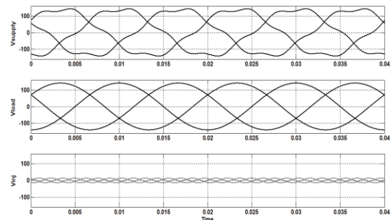
Fig. 3. Waveforms for the supply voltage, desired load voltage and the compensating voltage
