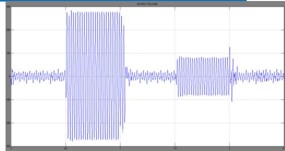
Fig.13 Simulated output wave form from the Compensating voltages generated by the DVR.
