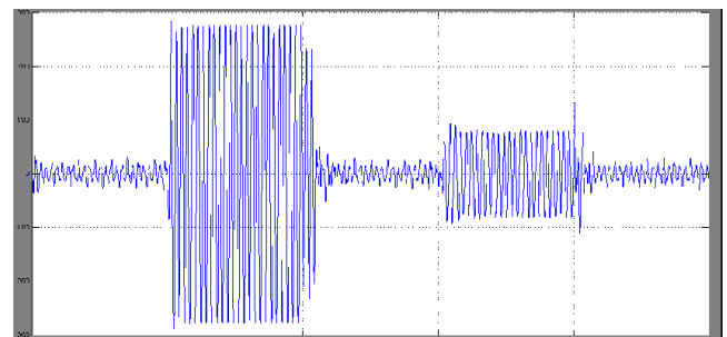
Fig.9 Simulated output wave form from the Compensating voltages generated by the DVR.
