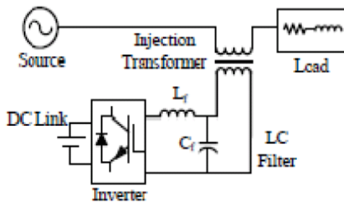
Fig. 1. Basic Components of a DVR
