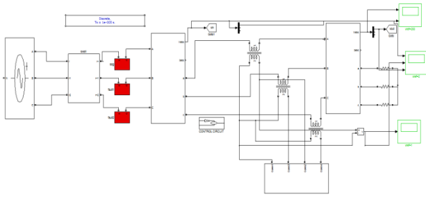
Fig.10 Matlab/Simulink model of fault and Swell generation and mitigated by Z-source DVR
