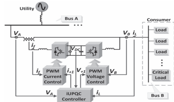
Fig 1 Modified iUPQC Configuration
