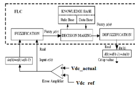
Fig.4. Block diagram of the Fuzzy Logic Controller (FLC) for proposed converter.
