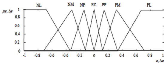
Fig.5. Membership functions for Input, Change in input, Output.
