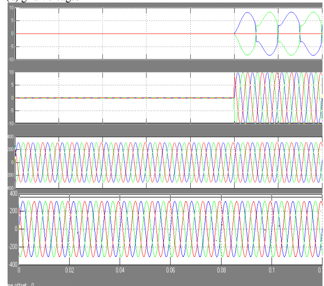
Fig 9 iUPQC transitory response during the connection of a two phase diode rectifier: (a) load currents, (b) source currents, (c) load voltages, and (c) source voltages.
