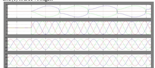
Fig 10 simulation wave form of iUPQC response at no load condition grid voltages V_A , load voltages V_B , and grid currents with fuzzy controller
