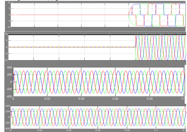
Fig 8 iUPQC transitory response during the connection of a three phase diode rectifier: (a) load currents, (b) grid currents, (c) load voltages and (d) grid voltages
