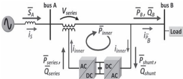
Fig.3. iUPQC power flow in steady-state
