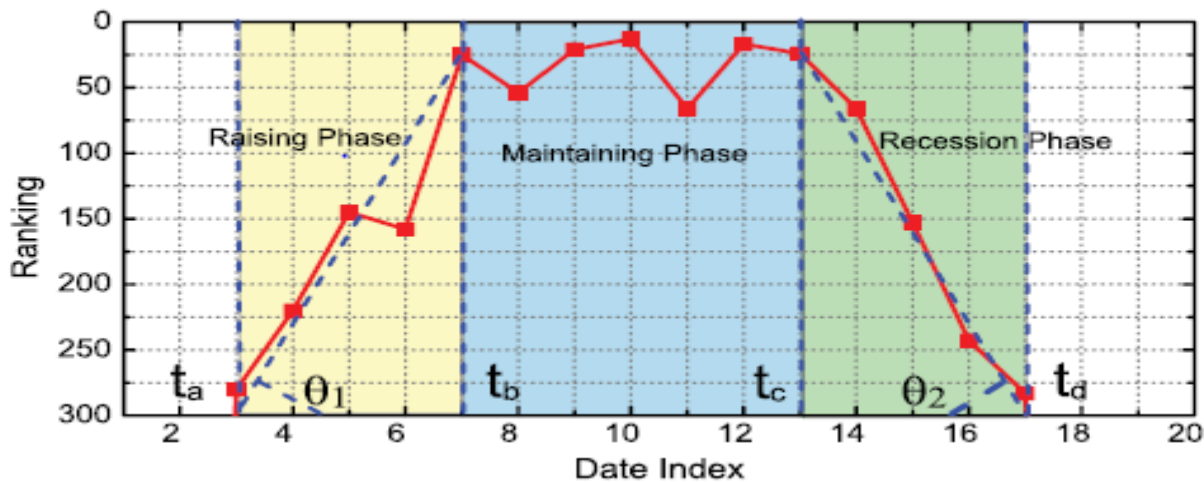
Fig2: Leaderboard (phases)
