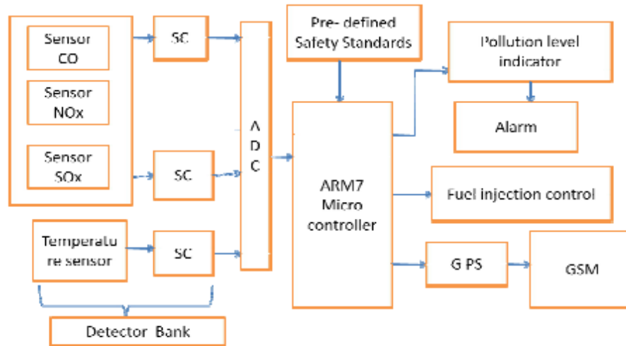
Figure: 1 schematic diagram of pollution monitoring
