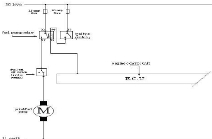
Figure: 2 Fuel pump wiring circuit
