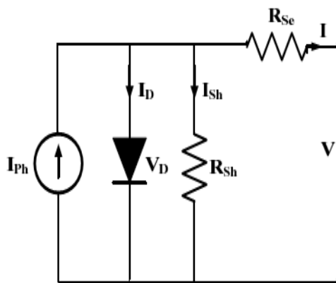
Fig.2. PV (Solar cell) modeling
