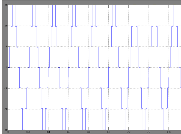
Fig 5 simulation wave form of conventional method seven level inverter
