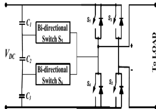
Fig.3. A single phase seven-level Modified PWM Inverter Implementing with a modified PWM inverter topology that uses only six switches. The system consists of a capacitor voltage divider, an H bridge and also a two bidirectional switches. In this paper we used a modified Pulse Width Modulating (PWM) technique. The system consists of a capacitor voltage divider, an H bridge and also a bidirectional switches. Switches are IGBTs with diode's. The triggering pulses for the six switches are generated by comparing three reference waves with the carrier wave. The reference signals and the carrier will have same magnitude and the frequency but each reference is shifted by value equal to carrier magnitude. The reference voltages are compared the carrier wave and firing pulses for the 6 switches are generated. The single H-bridge provides 3 level output. Remaining 4 levels (+V/3, +2V/3 and -V/3, -2V/3) are obtained by triggering S2 with S5&S6, S3 with S5&S6. The modified topology used for both standalone and hybrid systems that leads in low cost and less complexity.
