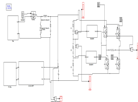
Fig.3. A single phase seven-level Modified PWM Inverter Implementing with a modified PWM inverter topology that uses only six switches. The system consists of a capacitor voltage divider, an H bridge and also a two bidirectional switches. In this paper we used a modified Pulse Width Modulating (PWM) technique. The system consists of a capacitor voltage divider, an H bridge and also a bidirectional switches. Switches are IGBTs with diode's. The triggering pulses for the six switches are generated by comparing three reference waves with the carrier wave. The reference signals and the carrier will have same magnitude and the frequency but each reference is shifted by value equal to carrier magnitude. The reference voltages are compared the carrier wave and firing pulses for the 6 switches are generated. The single H-bridge provides 3 level output. Remaining 4 levels (+V/3, +2V/3 and -V/3, -2V/3) are obtained by triggering S2 with S5&S6, S3 with S5&S6. The modified topology used for both standalone and hybrid systems that leads in low cost and less complexity.
