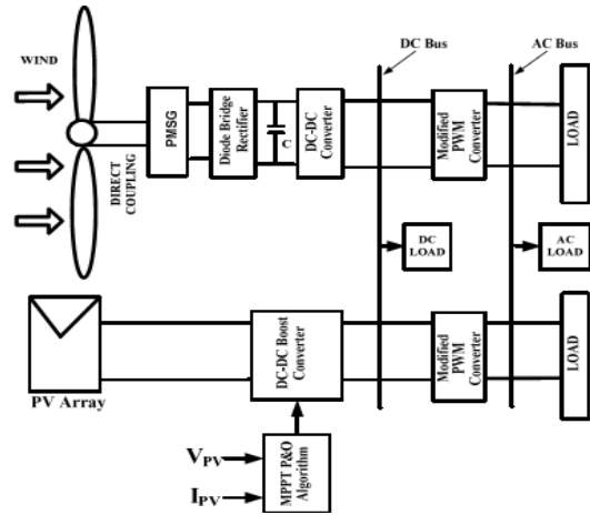
Fig.1. Block diagram of Implemented Hybrid System with Modified PWM converter Topology.
