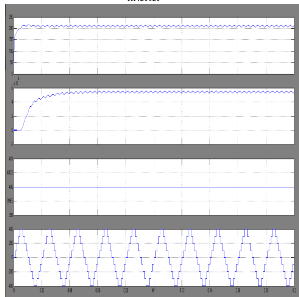
Fig 8 simulation wave form of proposed method of nine-level inverter output
