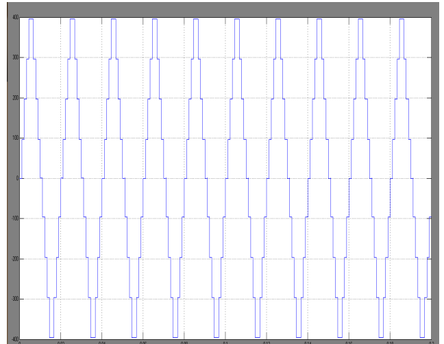
Fig 7 simulation wave form of proposed method of nine-level inverter
