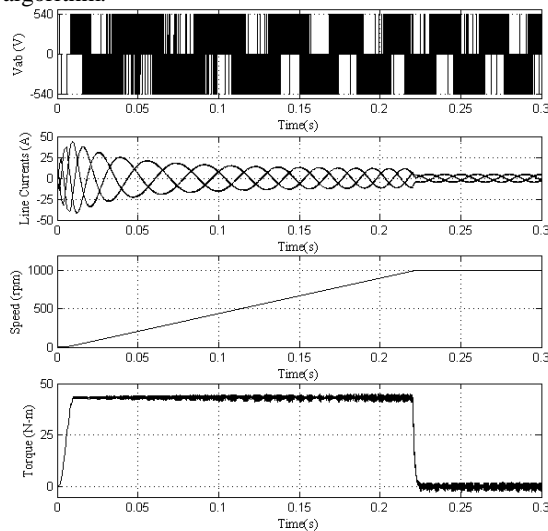
Fig. 5 starting transients of classical vector control algorithm based induction motor drive
