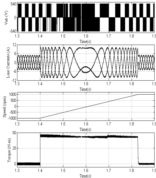
Fig. 16 Transients during the speed reversal (from -1000 rpm to +1000 rpm) for DSVM algorithm based vector controlled induction motor drive
