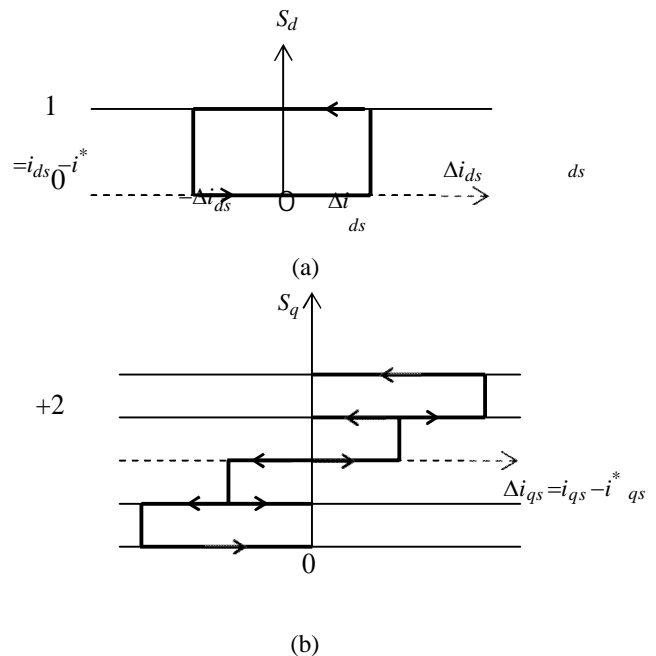
Fig. 4 (a) d-axis current controller (b) q-axis current controller
