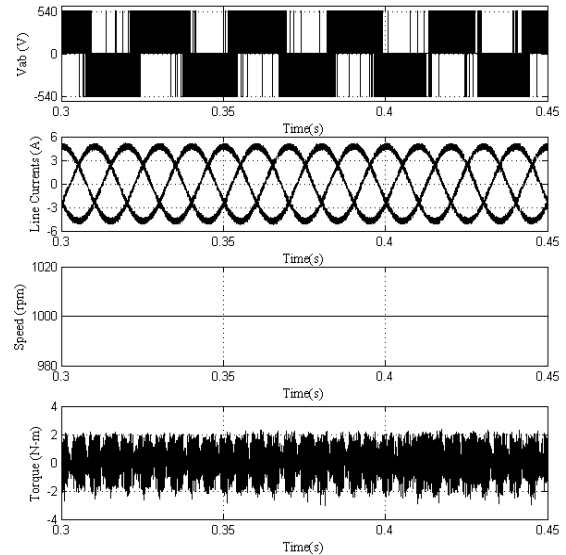
Fig. 6 steady state plots of classical vector control algorithm based induction motor drive
