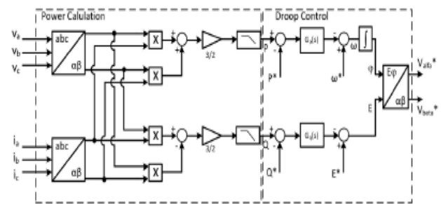
Fig. 4. Block scheme of classical droop control.
