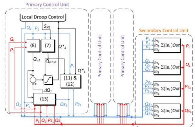
Fig. 8. Block diagram of developed reactive power sharing algorithm in real-time implementation.
