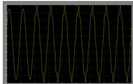
Fig 4: Grid current waveforms with DC component
