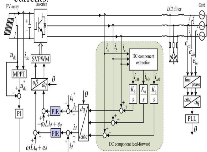
Fig 2: DC component minimization strategy based on dc component feed-forward and PIR controllers.
