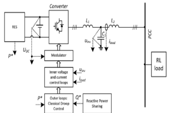
Fig. 3. Block scheme of control structure for one of the converters in islanded MG.
