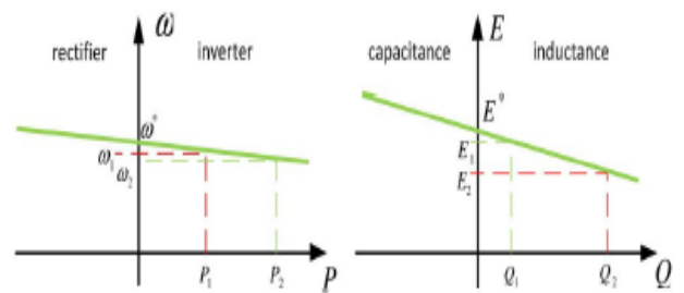
Fig. 2. P- \omega and Q-E droop characteristics.
