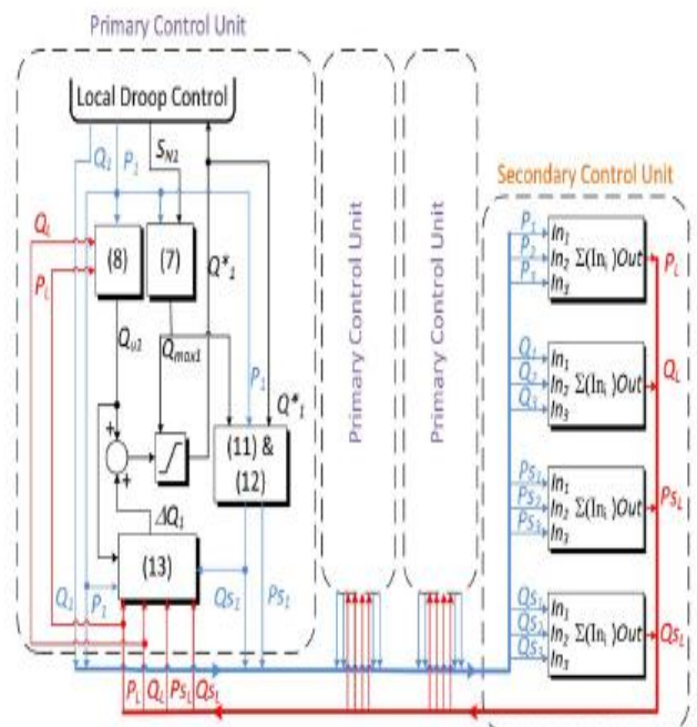
Fig. 8. Block diagram of developed reactive power sharing algorithm in real-time implementation.
