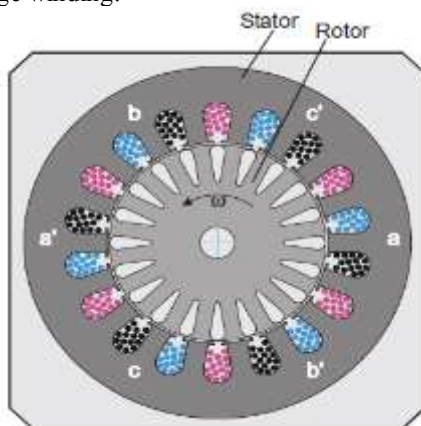
Fig 9 3-Phase AC Induction Motor
