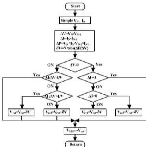
Fig.3 Flowchart of the variable step size INC MPPT algorithm
