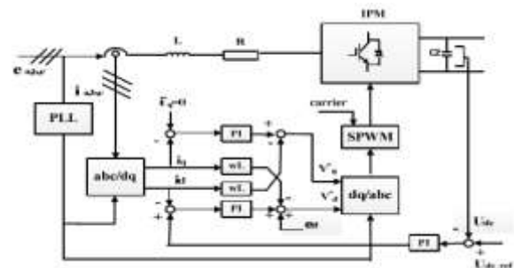
Fig.5 Control strategy of the bi-directional DC/AC converter
