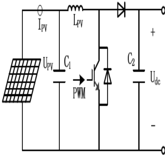
Fig.2 DC/DC converter of PV module with MPPT function
