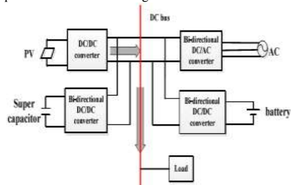
Fig.8 Power flow of mode I
