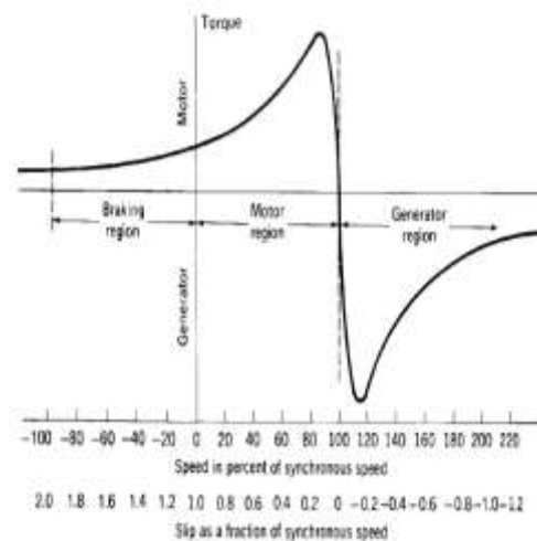
Fig 10 AC Induction Motor Speed-Torque Characteristic
