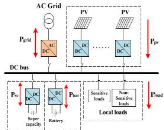
Fig.1. DC microgrid with hybrid storage system
