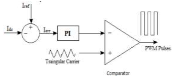
Fig. 3 Current Controller Block
