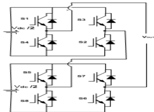
Figure.7. Five level CHB inverter
