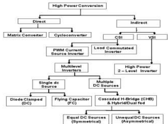
Fig.4 classifications of power converters
