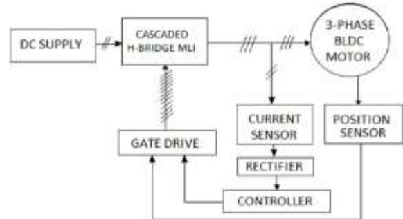
Fig.2 Current Controller of BLDC Motor with MLI
