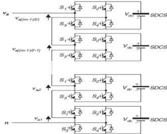
Figure 5. Single-phase structure of a multilevel cascaded H-bridge Inverter.
