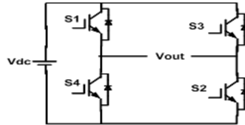
Figure 6. Full H-Bridge inverter Table I Switching table for Full H-Bridge inverter
