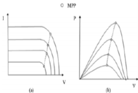
Fig1. (a) V-I characteristics (b) P-V characteristics of PV panel at different environmental conditions.
