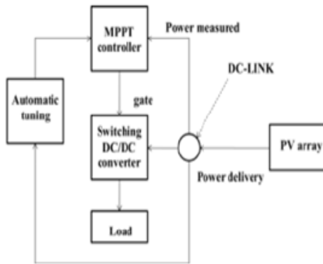
Fig2. Schematic representation of Adaptive Perturb and Observe method.
