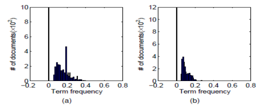
Fig. 2. Distribution of term frequency (TF) for (a) keyword "subnet", and (b) keyword "host".
