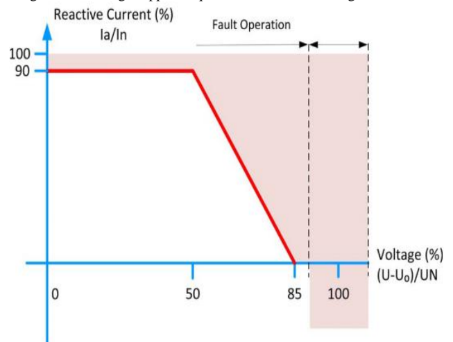
Fig.5. REE voltage support requirement in the event of grid fault.
