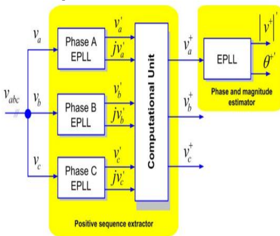
Fig.8. 3phEPLL block diagram.
