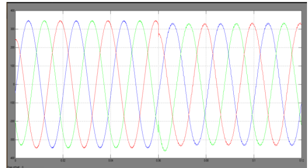
Fig.16 simulation wave form DSOGPLL harmonic, frequency, LLLG and unbalance condition
