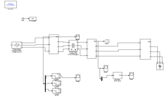
Fig 17 Matlab/simulation circuit of three-phase enhanced PLL (3phEPLL)
