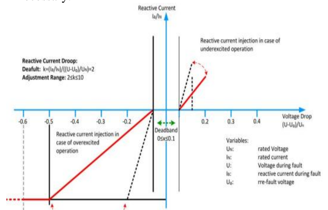
Fig.4. E-on voltage support requirement in the event of grid fault.
