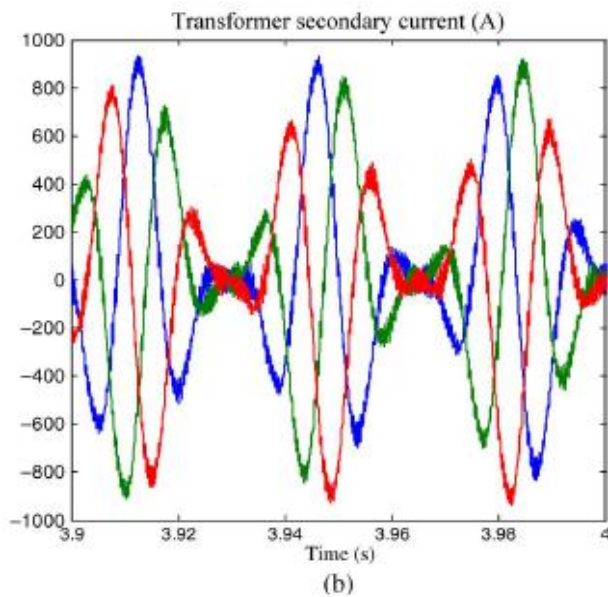
Fig.9. Inverter (transformer secondary) current with and without resonant controller applied: (a) without resonant controller and (b) with resonant controller.
