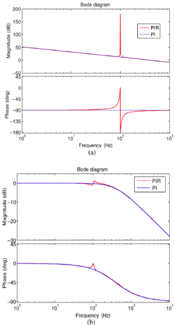
Fig. 8. Current-loop frequency response with PI and PIR controllers: (a) open loop frequency response and (b) closed-loop frequency response.
