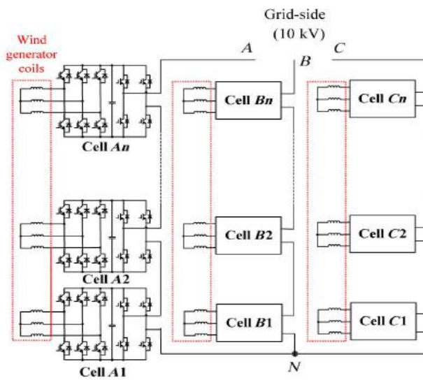
Fig.2. High-power, medium-voltage (10 kV) modular wind converter with generator-side isolation (converter type I).
