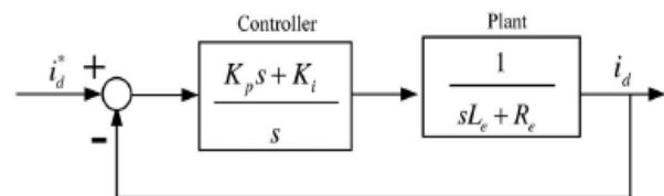
Fig.7. Current-loop diagram with a PI controller
