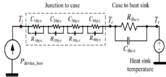
Fig.10. Thermal network to evaluate the device junction temperature.
