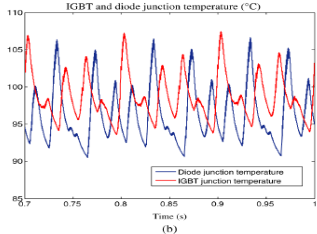
Fig.11. Inverter device (IGBT/diode) junction temperature variation: (a) without resonant controller and (b) with resonant controller.
