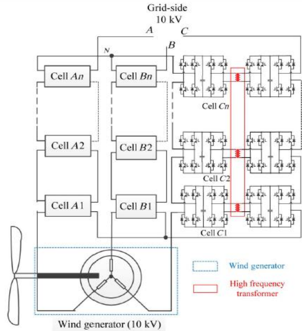
Fig.3. High-power, medium-voltage (10 kV) modular wind converter with high frequency transformer isolation (converter type II).
