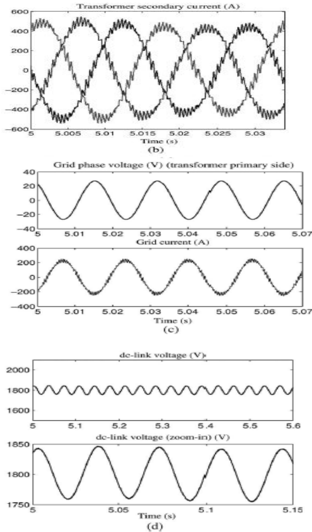
Fig. 12. Steady-state simulation results at wind speed of 12 m/s: (a) generator side converter output voltage and generator current, (b) transformer secondary winding current in a converter cell, (c) grid phase voltage and current, and (d) dc-link voltage and detailed trace.
