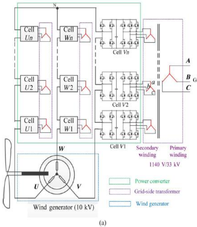
Fig.4. High-power, medium-voltage (10 kV) modular wind converter with grid side transformer isolation (converter type III): (a) generator and converter structure and (b) wind turbine electrical configuration.
