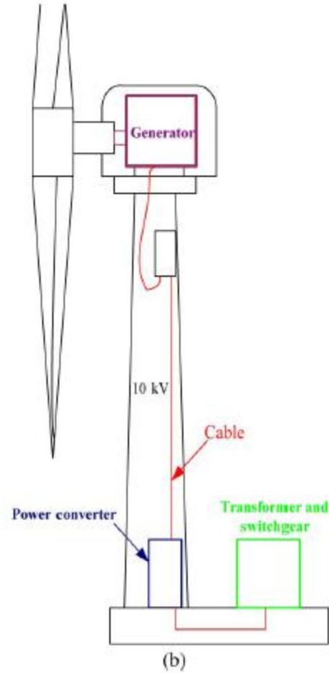
Fig.4. High-power, medium-voltage (10 kV) modular wind converter with grid side transformer isolation (converter type III): (a) generator and converter structure and (b) wind turbine electrical configuration.
