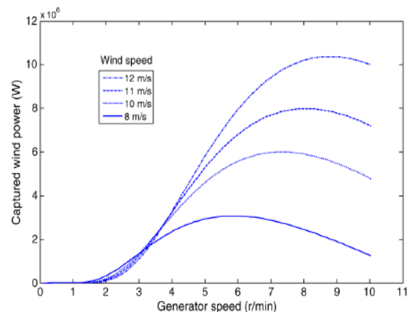
Fig.5. Variation of captured wind power with generator speed under different wind speeds.
