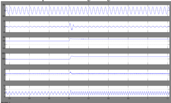
Fig.10. Test results of proposed BLDC motor drive showing dynamic performance during change in dc-link voltage from 100 to 150 V.
