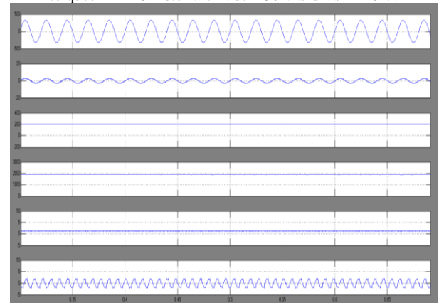
Fig.8. Test results of proposed BLDC motor drive At rated load torque on BLDC motor with Vdc = 200 V and Vs = 220 V.
