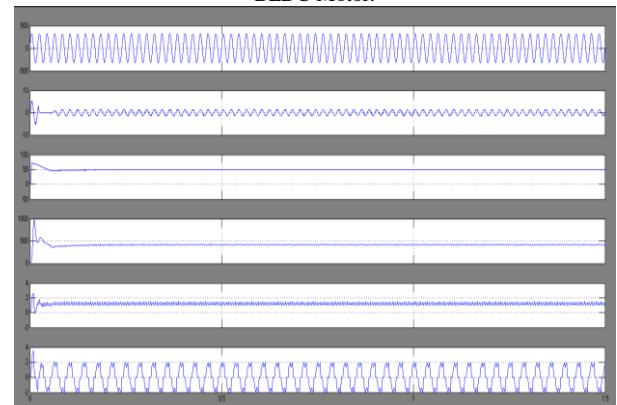
Fig.7. Test results of proposed BLDC motor drive At rated load torque on BLDC motor with Vdc = 50 V and Vs = 220 V.
