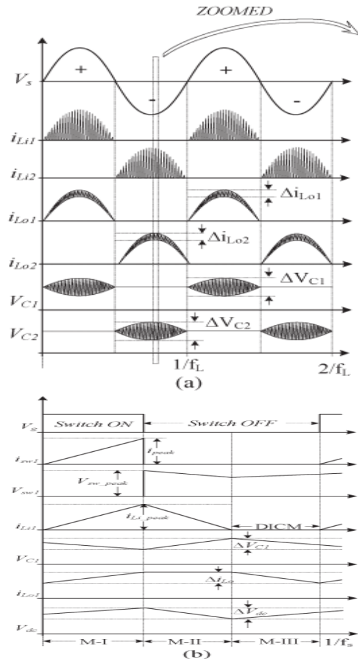
Fig. 4. Waveforms of BL-Luo converter during its operation for (a) complete line cycle and (b) complete switching cycle.
