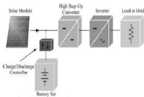
Figure1: Typical photovoltaic system
