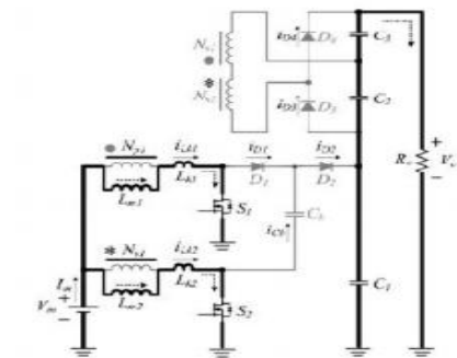
(a) Mode-1 [t0, t1].
