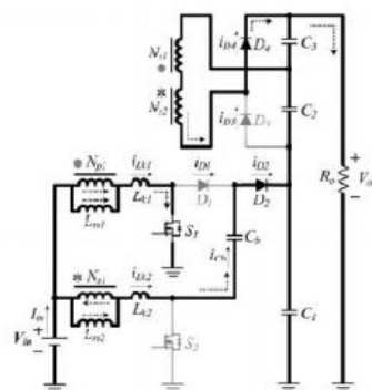
(b) Mode-2 [t1, t2]
