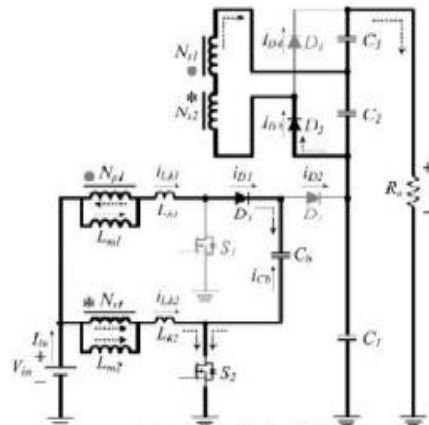
(e) Mode-5 [t4, t5].
