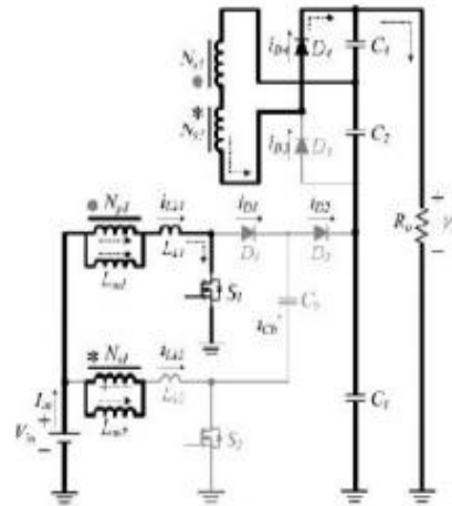
(c) Mode-3 [t2, t3].
