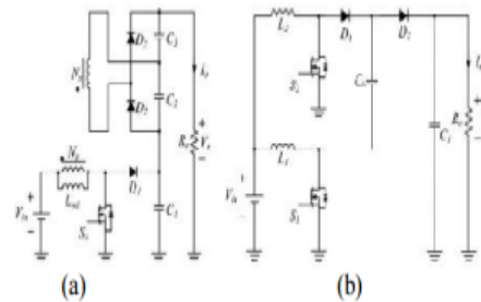
Figure 2: High step-up techniques based on a classical boost converter. (a) Integrated fly back-boost converter structure. (b) Interleaved boost converter with a voltage-lift capacitor structure
