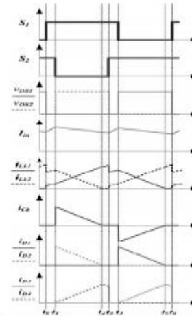
Figure 4: Steady waveforms of the proposed converter at CCM.
