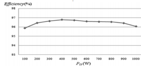
Figure 9: Measured efficiency of the proposed converter.
