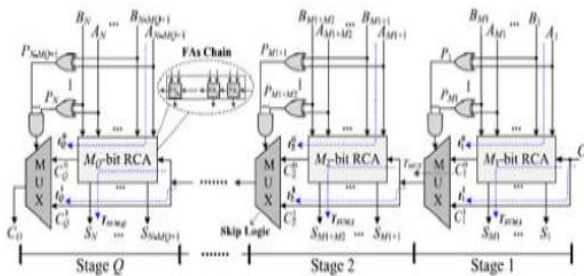
Figure 2: Structure of conventional CSKA
