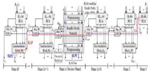
Figure 5: Structure of Modified CSKA
