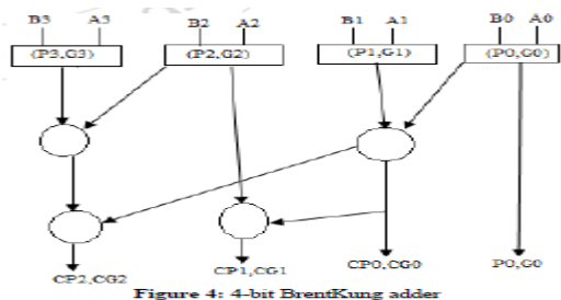
Figure 4: 4-bit BrentKung adder
