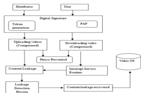
Fig.3. Working flow of proposed approach
