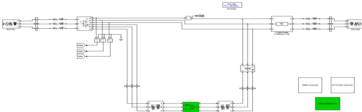
Fig. 3 Power System with UPFC
