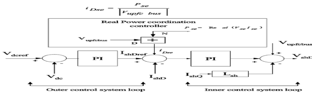
Fig.2. D-axis shunt converter control system with real power coordination controller.
