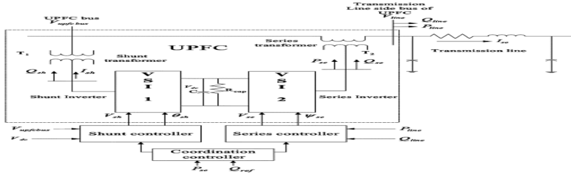
Fig.1 UPFC connected to a transmission line
