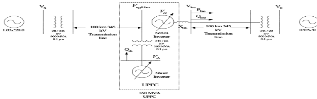
Fig. 3 Power System with UPFC
